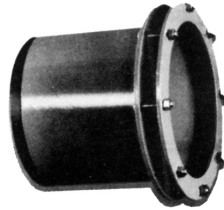
9" long. Male weld-on x bolt-on coupler
